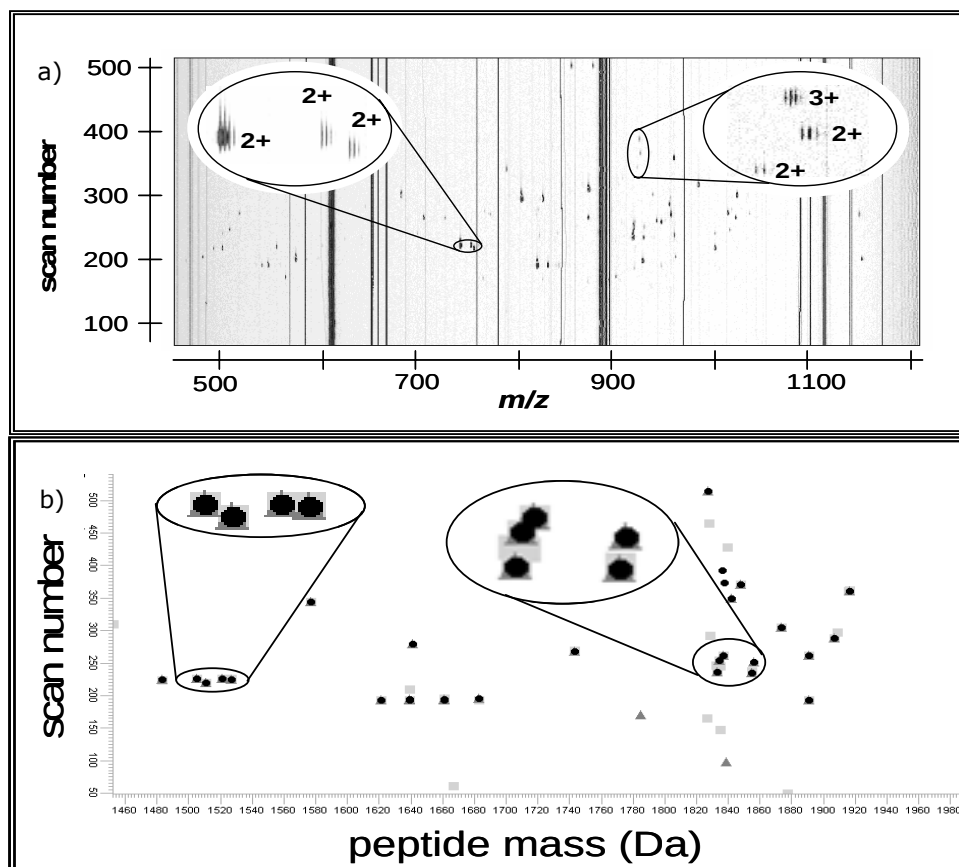
Figure 5.4. a) NanoLC-FTICR-MS measurement of a trypsin digested cerebral spinal fluid (CSF) sample displayed with the AWE3D software. The m/z -values are plotted on the x-axis, the scan numbers (linear with nanoLC retention times) on the y-axis and the peak intensities on the z-axis (out-of-plane). b) Visualization of a processed nanoLC-FTICR-MS measurement of a digested cerebral spinal fluid (CSF) sample. The peptide masses are plotted on the x-axis (from 1450 to 1980 Da) and the scan numbers (corresponding to retention time) on the y-axis (50-450). A peptide mass is visualized provided that it is detected in at least 3 sequential scans with a mass precision of 0.05 Da (see methodology). Here, different processing results are overlaid in one plot, i.e. no apodisation on the raw data (light grey squares), apodisation and AMOLF isotope cluster identification (grey triangles) and apodisation and Senko isotope cluster identification (black circles). The inserts show the similarity between AMOLF and Senko cluster identification results ( i.e. each triangle is overlapped by a circle). However, without apodisation additional clusters are detected or the cluster is observed at a slightly different peptide mass.
