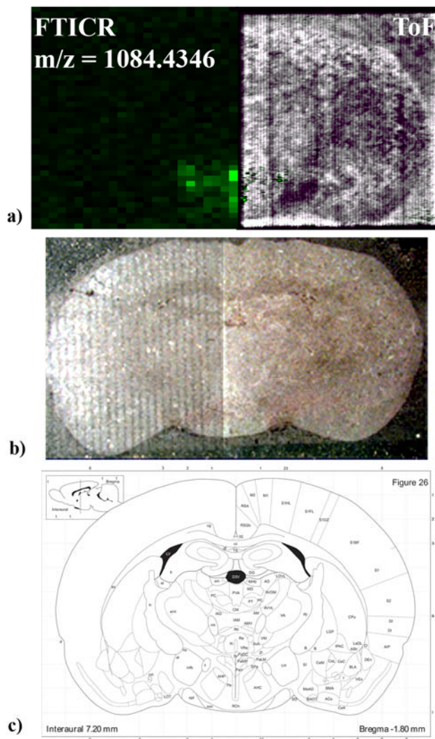
Figure 4.4. FTICR (left) and TOF (right) images of a) the distribution of Vasopressin m/z = 1084.44 on the brain section in green. For clarity in the right hand side TOF image the vasopressin distribution is overlain on the total ion image in black and white. b) Optical image with FTICR-MS laser tracks on the left clearly visible. c) Schematic representation of the anatomy of the rat brain tissue section with the specification where the tissue was taken from the brain.
