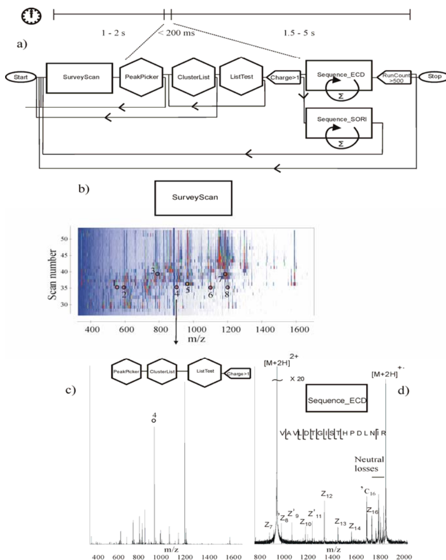
Figure 3.4. a) Workflow of automated ECD experiment b) 3D visualization of the SurveyScan for tryptic digested savinase (x = m/z, y = scan number, z = intensity); 1-AQSPWGISR (z = +2) 2-NPSWSNVQIR (z = +2) 3-NTATSLGSTNLYGSLVNAEAATR (z = +3) 4-VAVLDTGISTHPDLNIR (z = +2) 5-GVLVVAASGNSGAGSISYPAR (z = +2) 6-AQSPWGISR (z = +1) 7-NTATSLGSTNLYGSLVNAEAATR (z = +2) 8-NPSWSNVQIR (z = +1) c) selected spectrum –of 61 recorded- from SurveyScan d) selected ECD spectrum 4-VAVLDTGISTHPDLNIR (z = +2).
