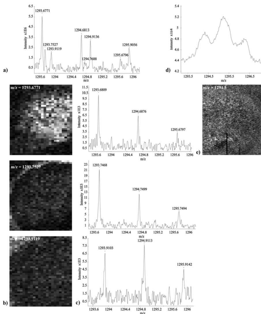
Figure 4.3. a) Selected region of the FTICR summed spectrum of half of the rat brain tissue section b) FTICR selected ion images of the first isotope of three different compounds c) Region of interest analysis reveals the spectrum of each individual component d) Selected region of the summed spectrum of half of the rat brain tissue section e) The TOF selected ion image of m/z = 1294 . Due to a technical problem a part of a line scan of TOF experiments is not present in the selected ion images.
