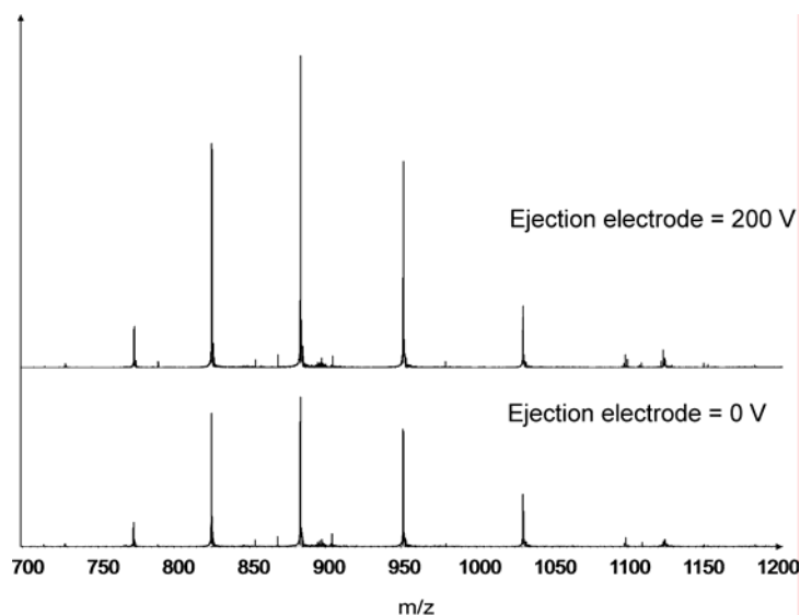
Figure A1.7. Experimental mass spectra of cytochrome c when 200 V (upper figure) and 0V (lower figure) were applied to the ejection electrodes of the curved ejection electrode configuration. The arbitrary y-scales on both figures are identical.
