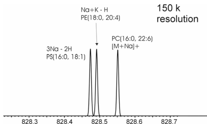
Figure 2.9. Use of MS/MS to obtain images of specific lipids a) and theoretical high mass resolution FTICR analysis of the same compounds. Note the DHB cluster ion is not in the m/z window of b) as its mass is too far away (easily resolvable). Taken from reference 79.
