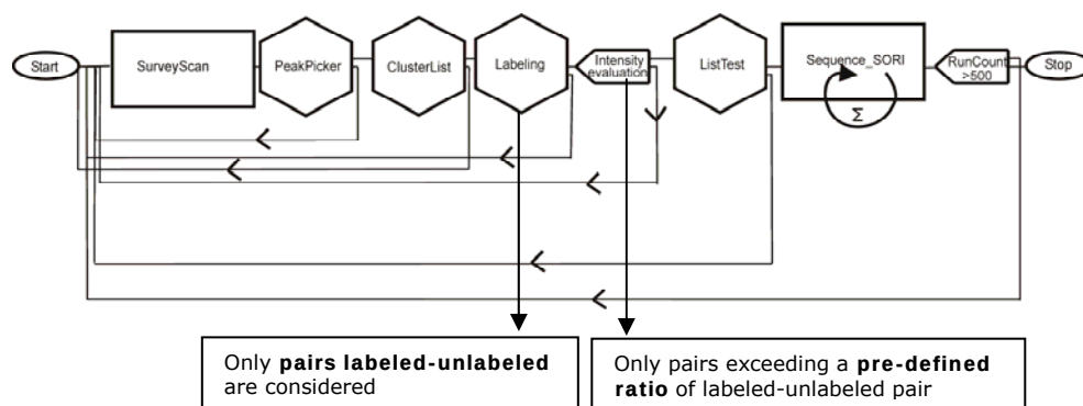
Figure 3.6. Workflow of automated targeted on-the-fly selection of labeled peptides.
